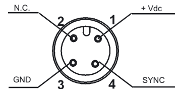
EMITTER (TX)
