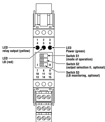
STI Intrinsic Safety Barrier
